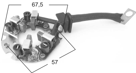
P2255C ARR. MITSUBISHI CHRYSLER, DODGE, NISSAN. 4.5 x 11 x 19 (M649T01271 Md611217) (colilla corta)
