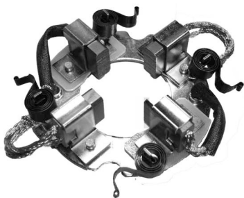
P2284C ARR. LUCAS M50, M127 9 x 20 x 24
