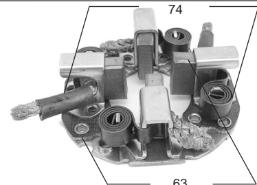
P2239C ARR. MITSUBISHI, MAZDA, NISSAN, DATSUN. 7x18x18.5 12v. (M649T05072 ME700127) P2239C/24 IDEM 24v. (M649T05072 ME700140)
