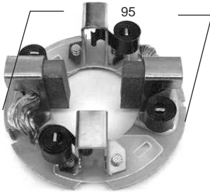
P2370C ARR. NIPPONDENSO, CATERPILLAR, CASE, CUMMINS, ISUZU. 10 x 30 x 20 (028510-0880 181118-043-0 28140-1310A)
