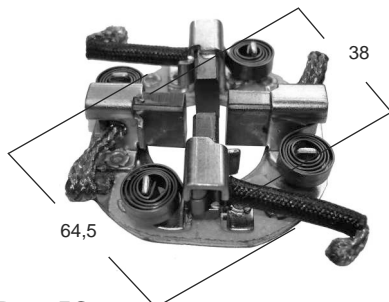
P2235C ARR. MARELLI, FIAT PALIO - SIENA, 6 x 14.8 x 19
