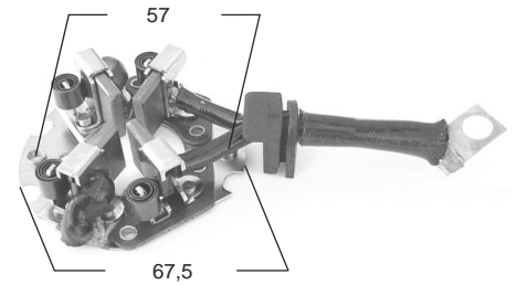
P2257C ARR. MITSUBISHI, CHEVROLET, FORD, SUZUKI. 4.5 x 18 x 17 12v. (F32Z-11061-B SBE-342 835 036 71-colilla corta)
