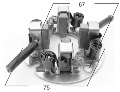
P2252C ARR. NIPPONDENSO, ISUZU, CHEVROLET, DODGE 7.8 x 25 x 15
