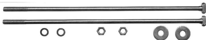
T2189 ARRANQUE TIPO GAREF FIAT 128/DUNA/UNO, PEUGEOT, DODGE 1500 M5X188MM. CABEZA MARTILLO (Cant. 2)
