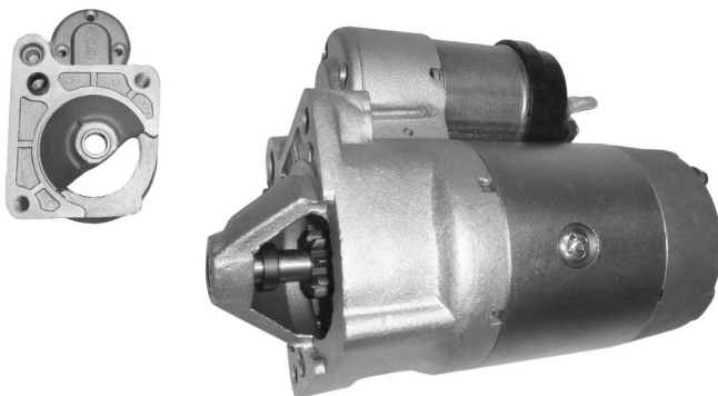
301163 RENAULT 9, 11, 12, 18 Y 19 MOTOR 1600 CC 12V-Z9-Ø25
