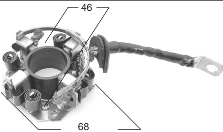
P2248C ARR. DELCO CHEVROLET BLAZER 6 x 19 x 16 (10475602)
