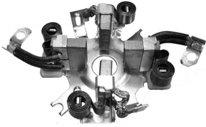
P2279C ARR. MARELLI, FIAT, MT 67 8 x 25 x 23
