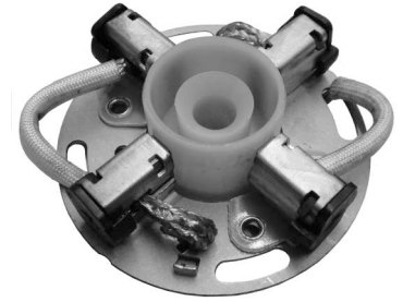
P2310C ARR. VALEO, RENAULT, PEUGEOT DIESEL, (ORIGINAL) 7 x 14 x 14
