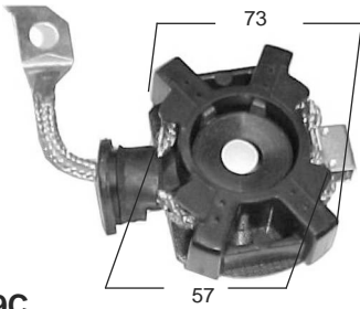
P2309C ARR. MOTORCRAFT, ESCORT, FIESTA, KA, F100, MONDEO 4.6 x 16 x 14 (E90Z-11061A/B/C)
