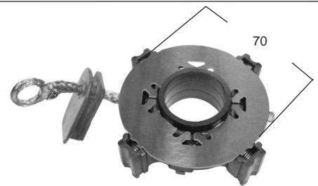
P2371C ARR. VALEO, CHEVROLET, PEUGEOT, RENAULT 6.5 x 8 x 11 (4 carb., colilla 38 mm) (D7EUF1171/4) (594351)
