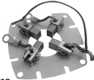
P2172C PORTA ESCOBILLA ARR. 6.5 x 9.6 x 17
