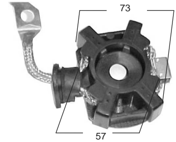
P2308C ARR. MOTORCRAFT, FORD MONDEO 4.6 x 16 x 14 (F3RZ11002C)
