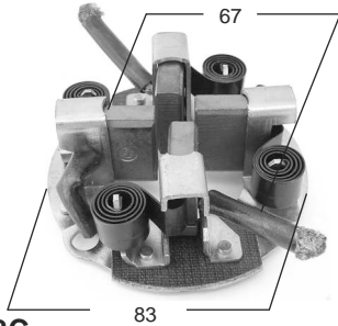
P2253C ARR. NIPPONDENSO, KUBOTA, TOYOTA, KOMATSU 7.8 x 25 x 21 (28140-77090)
