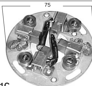
P2211C ARR. VALEO, RENAULT 19, EXPRESS, CLIO DIESEL, PEUGEOT 205/206/306/405 7 x 13 x 18
