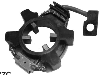
P2377C ARR. MOTORCRAFT, FORD EURO 4.8 x 13 x 12 12v.
