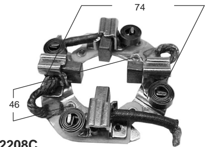
P2208C ARR. MARELLI, FIAT UNO, DUNA, RENAULT 11/12/18/19/21, TRAFIC 7 x 13 x 18 (F3RZ-11002C - F3RZ11061C)
