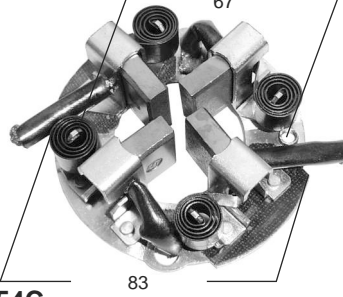
P2254C ARR. NIPPONDENSO, KUBOTA, TOYOTA, CASE. 7.8 x 25 x 21 24v(028510 0500)
