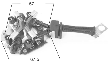
P2258C ARR. MITSUBISHI, CHEVROLET, FORD, SUZUKI. 4.5 x 18 x 17 12v. (colilla larga)
