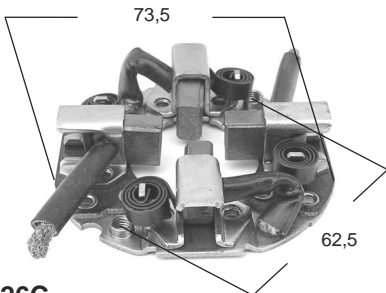
P2226C ARR. MITSUBISHI, CORSA, ISUZU, NISSAN, PICK UP, LUV, SENTRA. 7 x 12 x 17.5 (M649X20471 ME701467)
