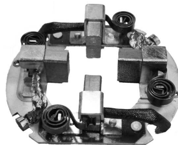
P2277C ARR. HITACHI NISSAN, ISUZU 9 x 19.5 x 22
