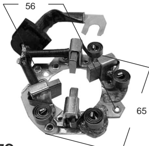
P2137C ARR. HITACHI, ESCORT, POLO POINTER, R19 - 4.5 x 14 x 15.5 (352 58 566)
