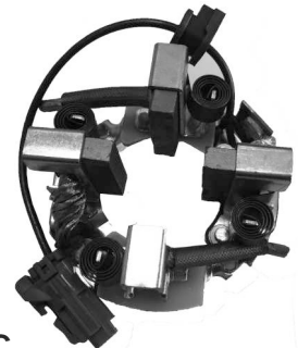
P2181C ARR. MITSUBISHI VOLVO: B12, FM12, FH 12, 8 x 30 x 18,2 24v.
