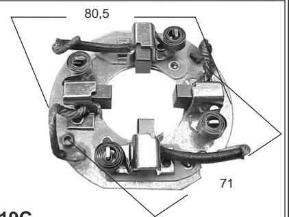
P2219C ARR. NIPPONDENSO, HONDA, ISUZU, DATSUN 6.8 x 11 x 19
