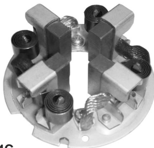
P2364C ARR. NIPPONDENSO CATERPILLAR, CUMMINS CASE 24v. 10 x 30 x 21
