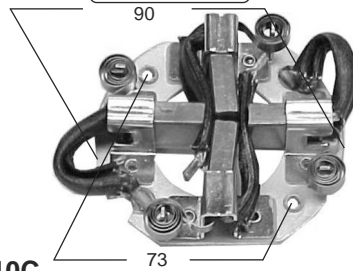
P2210C ARR. INDIEL M50, M115, M127, FORD CON MOTOR MAXION - MWM 9 x 20.5 x 24.5
