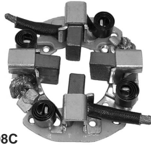
P2408C ARR. NIPPONDENSO, CHRYSLER, DODGE, ISUZU, TOYOTA 7 x 16 x 15.5 24v.
