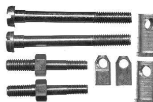
T2215 KIT ARRANQUE TIPO BOSCH / WAPSA, GOL DIESEL, SENDA DIESEL, SAVEIRO DIESEL (Cant. 1)
