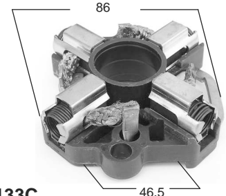
P2133C ARR. FORD, M.BENZ, NISSAN, OPEL, BMW 7.5 x 18 x 19 (9 003 334 314/1 004 112 906/907) GIRO HORARIO
