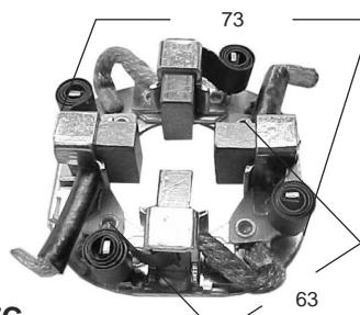
P2217C ARR. NIPPONDENSO, MITSUBISHI, MAZDA, HONDA, ISUZU 8 x 19 x 18
