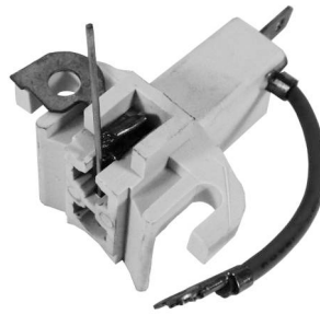
P7126 ALT. FORD 70 - 100 AMP 4 X 7.6 X 13
