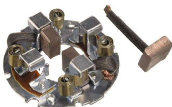
12138 - DELCO REMY
